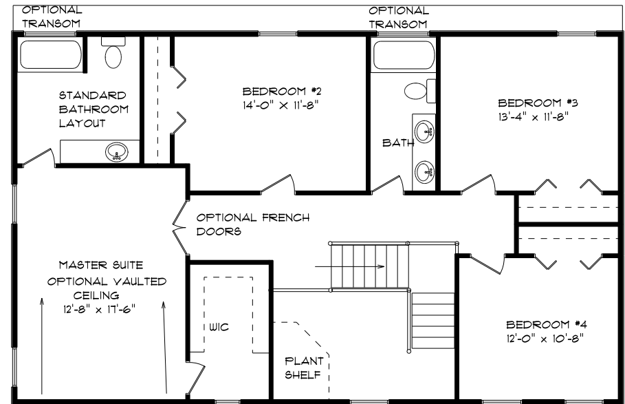
OPTION #2 SECOND FLOOR PLAN
